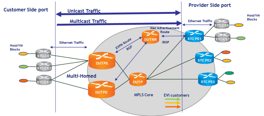
Figure 1: EVPN topology diagram
