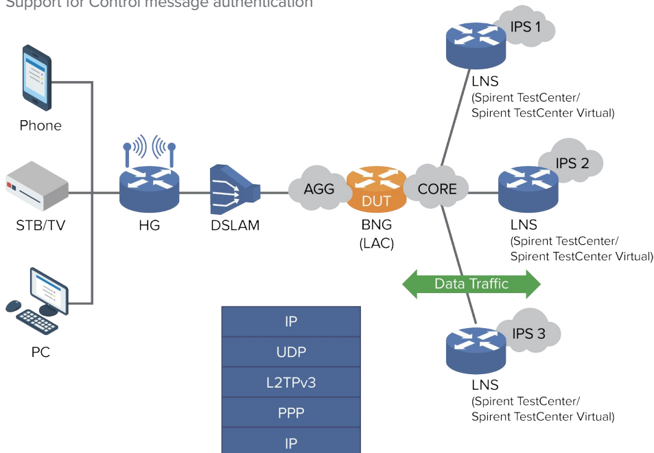
L2TPv3 with LNS Emulation
